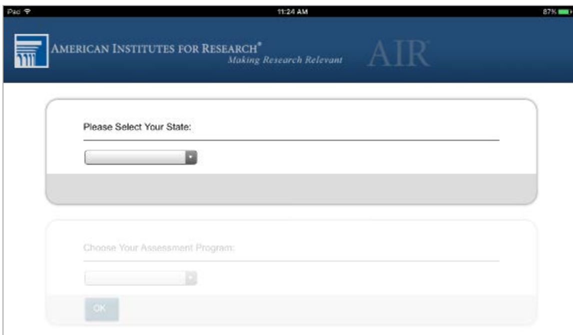
Figure 16. AIRSecureTest Launchpad
